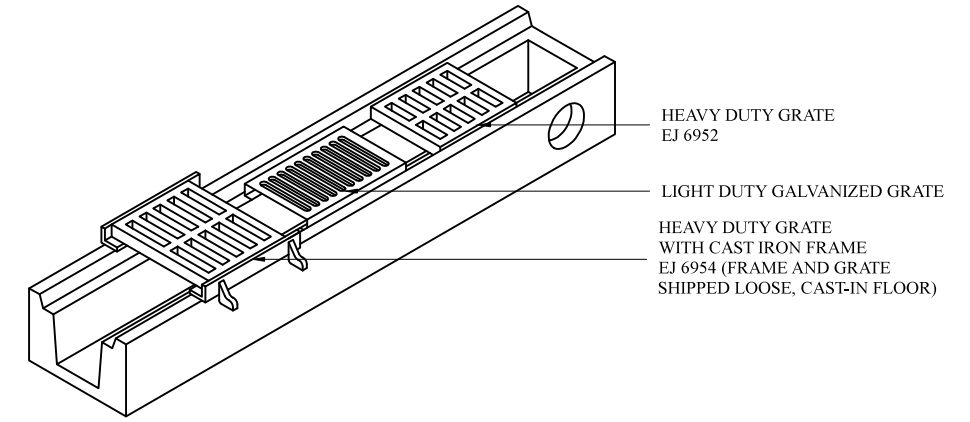
ISOMETRIC VIEW
